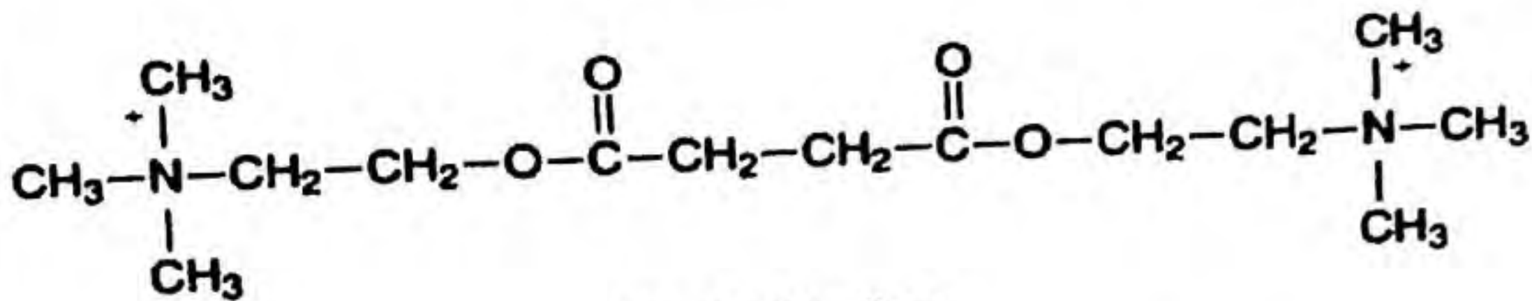
Succinylcholine
